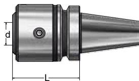
MAS 403 BT
