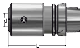
HSK63 DIN69893
